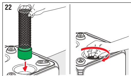
Fig. 22: Screw the new ionizing generators into place by acting again on the glass surface that can be reached by hand through the special slots.
